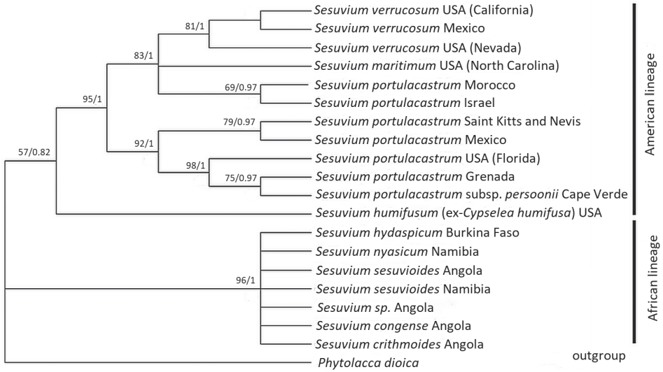
Figure 5. Phylogenetic relationships of perennial Sesuvium species from ML analysis of combined plastid sequences (rps 16 intron, trnL-trnF, atpB-rbcL, 1377 bp in total). The tree is drawn to scale, with branch lengths measured in the number of substitutions per site. ML bootstrap support/BI posterior probabilities are specified at the branch nodes (not shown when <50%).
