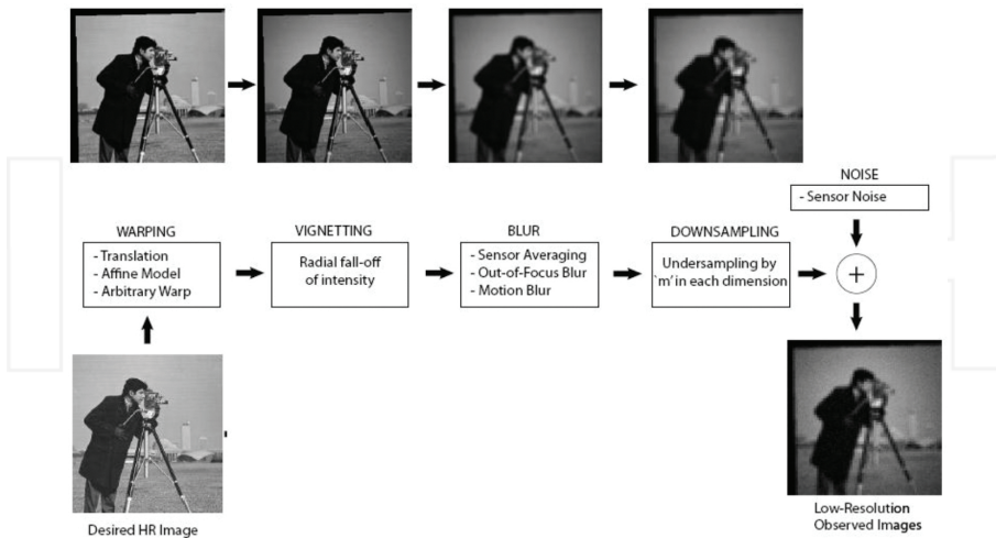
Figure 7. General observation model proposed in Ref. [5].
