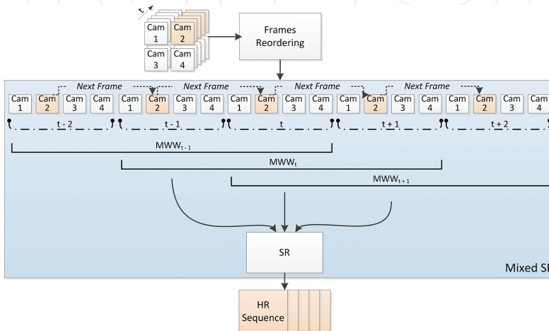
Figure 16. Mixed SR method [22].
