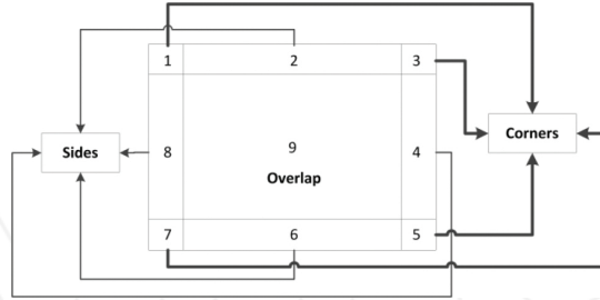
Figure 12. Frames division of the MC array in Overlap + Borders mode [22].
