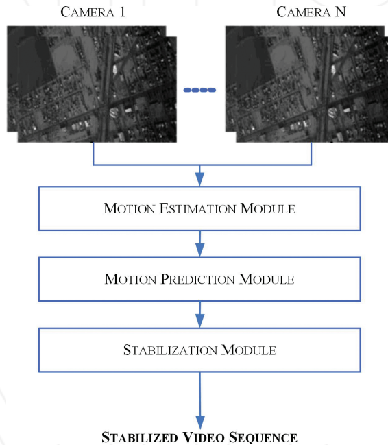
Figure 5. Video stabilization algorithm flow chart [14].
