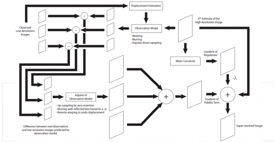
Figure 8. Single iteration in regularized super-resolution restoration [5].
