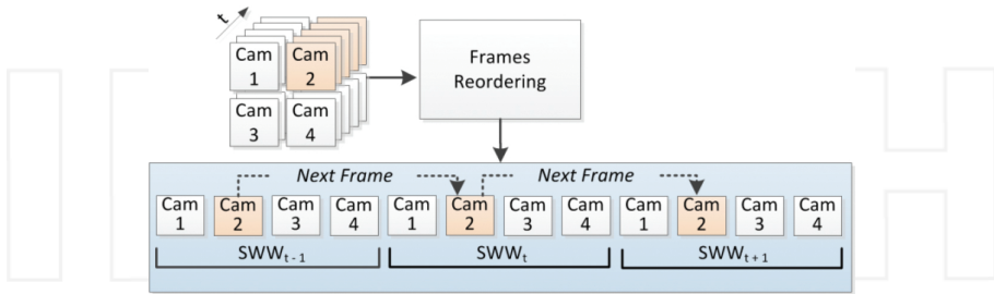
Figure 14. Frames reordering process [22].
