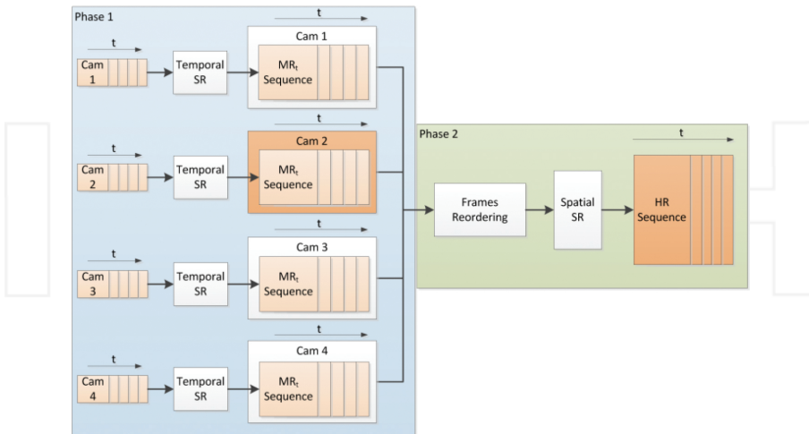
Figure 13. Temporal-spatial SR method [22].
