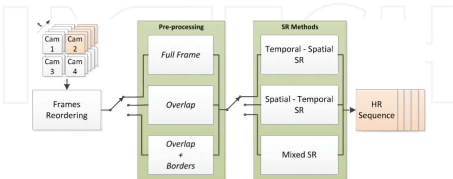
Figure 10. General scheme showing preprocessing modes and SR methods [22].
