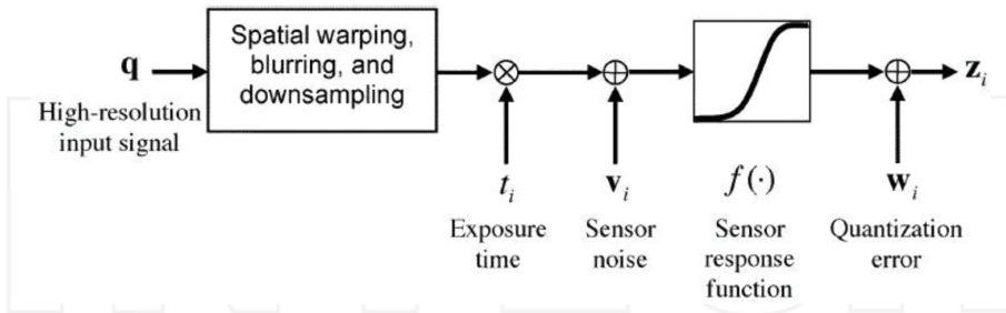
Figure 6. SR algorithm proposed in Ref. [20].
