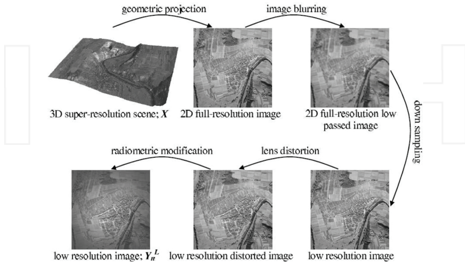
Figure 9. 3D-SR observation model [9].
