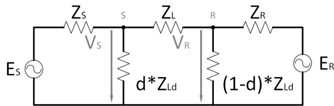
Figure 1. Modified power line model.
